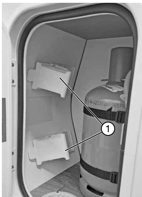
Chocks in the gas-bottle container
